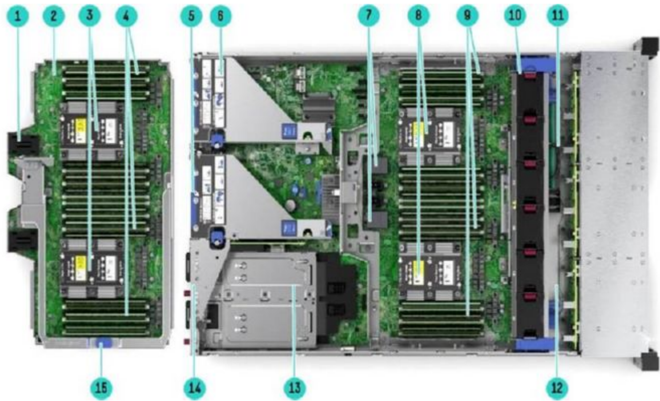
View: DL560 Gen10 with upper CPU mezzanine tray
