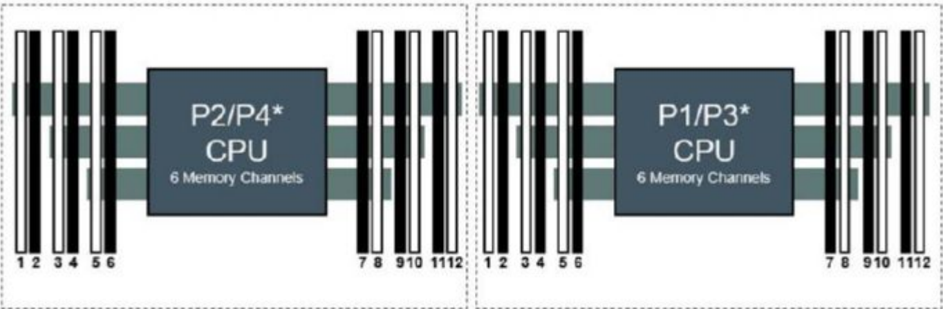
HPE ProLiant Gen10 DL360/ DL380/ DL560* Servers 2 Slots per Channel Notes:*HPE ProLiant DL560 is a 4 socket server (uses P3, P4)
