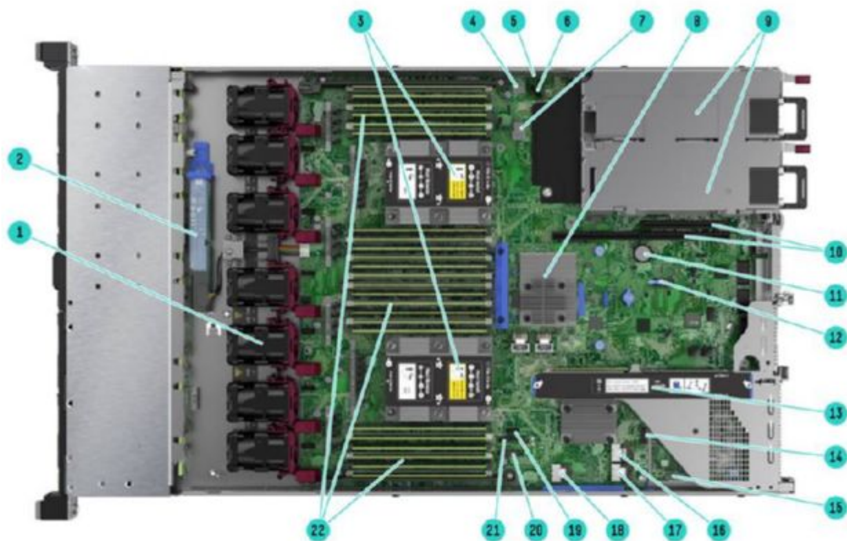
Internal View - Standard for all DL360 Gen10
