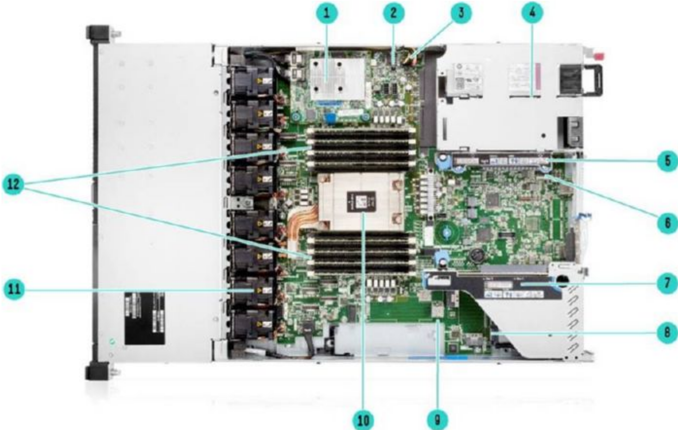
Internal View 8SFF chassis
