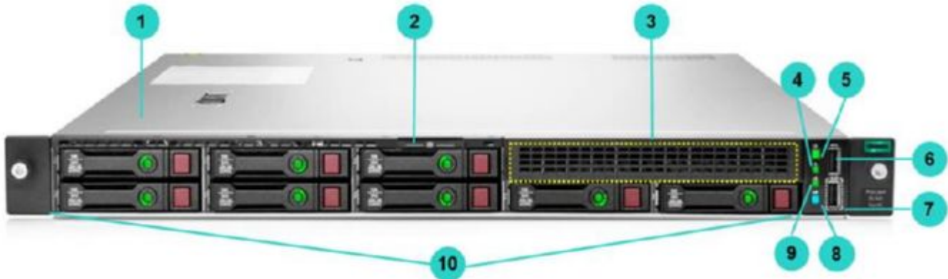
8 SFF chassis - Front View
