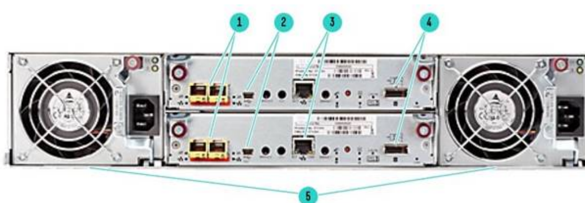
HPE MSA 1050 SAN Storage - Rear View
